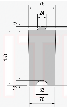
Section Profile (scale 1:5)
