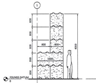
TYPICAL SECTION 01 - PERIMETER WALLS
