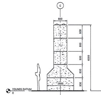
TYPICAL SECTION 02 - DIVIDING WALLS
