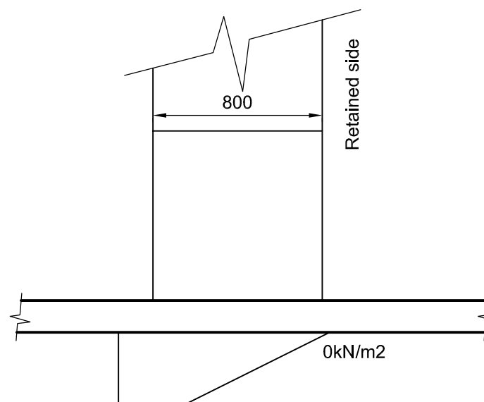
Bearing Pressure Beneath 150mm slab
