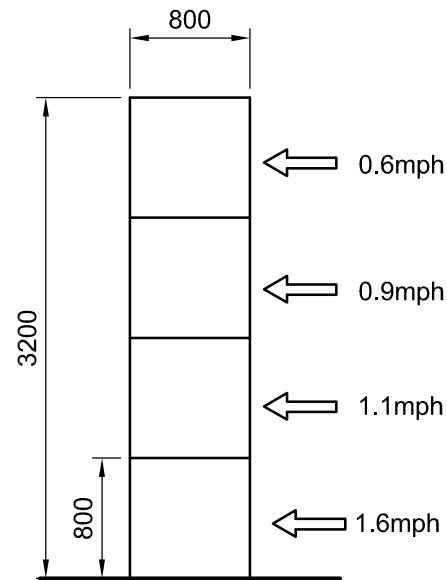
Max. Permissible Impact Loads
