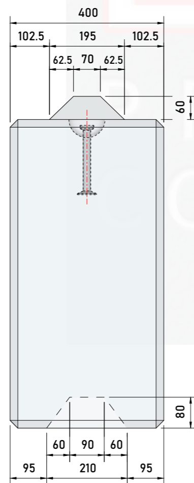
FRONT
