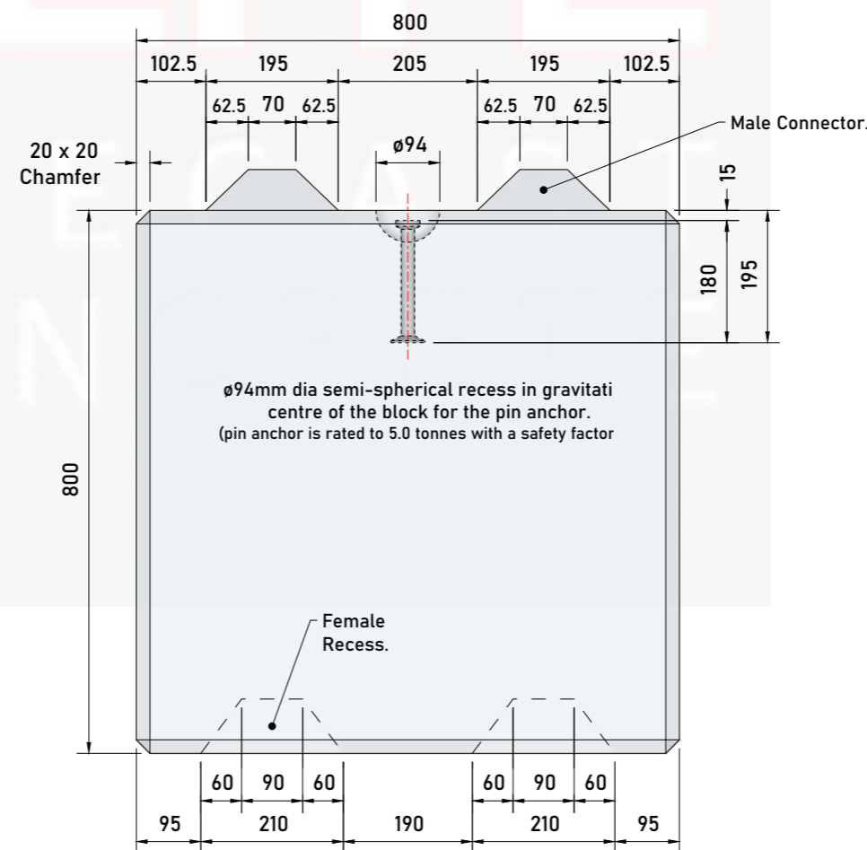
SIDE
