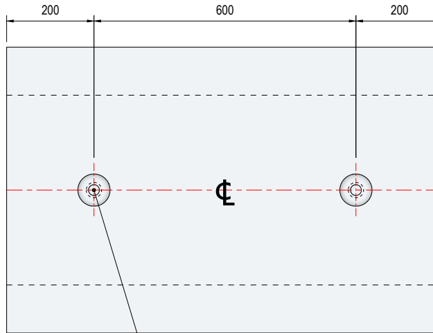
2 x 2.5t Lifting Pin x 55mm long (factor of safety x 3).
