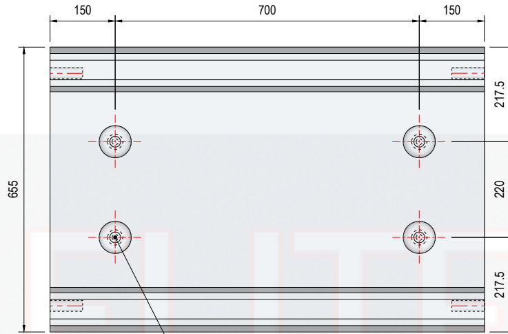
4 x 2.5t Lifting Pin x 55mm long (factor of safety x 3).
