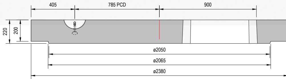
Section on Arrow A - A
