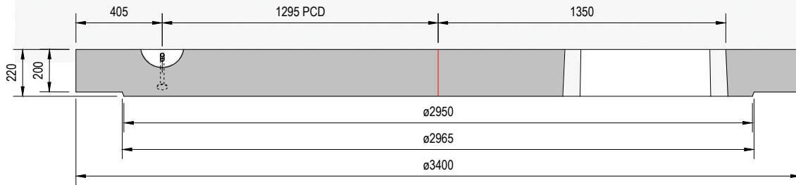
Section on Arrow A - A
