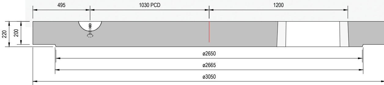
Section on Arrow A - A
