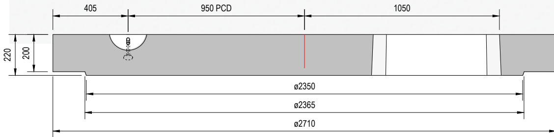
Section on Arrow A - A
